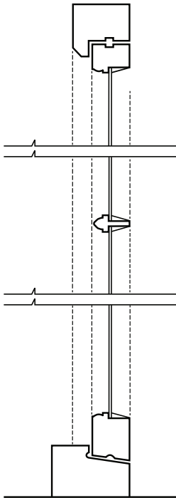
Typical Vertical Section through a Casement Window (Scale 1:5)
